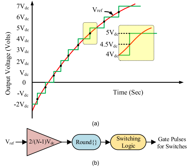
FIGURE 6. Nearest level control with. (a) sampled reference signal and. (b) implementation of NLC.
