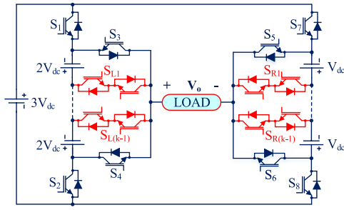
FIGURE 5. Extension III of the basic unit.
